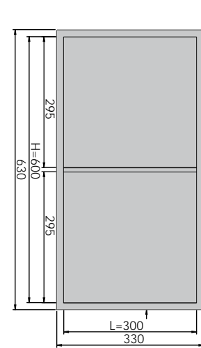
Model 30x60 cm
